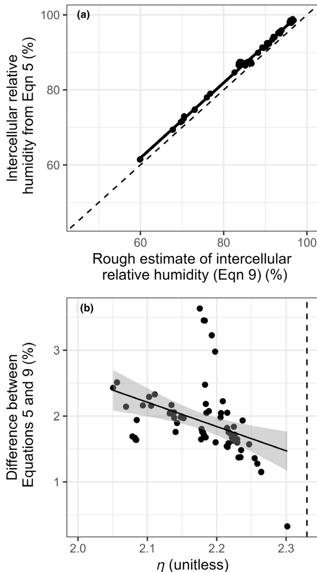
Fig. 6 The approximate solution ('rough estimate') of intercellular relative humidity (Eqn 9) closely tracks the full solution (Eqn 5), and the difference between those two estimates is largely determined by the value of \eta (the proportion by which helox increases total vapor conductance). In (a), the dashed line is 1 : 1, and the solid line is a linear fit ( y = 1.007 \cdot x + 0.007 ; r^2_{\text{adj}} = 0.9943 , P < 2.2 \times 10^{-16} ). In (b), the dashed vertical line is at \eta = 2.33 (the theoretical value in the limit of zero boundary layer resistance and zero cuticular conductance), and the solid line is a linear fit, with the shaded region indicating 95% confidence intervals ( y = -0.065 \cdot \eta + 0.009 ; r^2_{\text{adj}} = 0.329 , P < 0.001 ).
