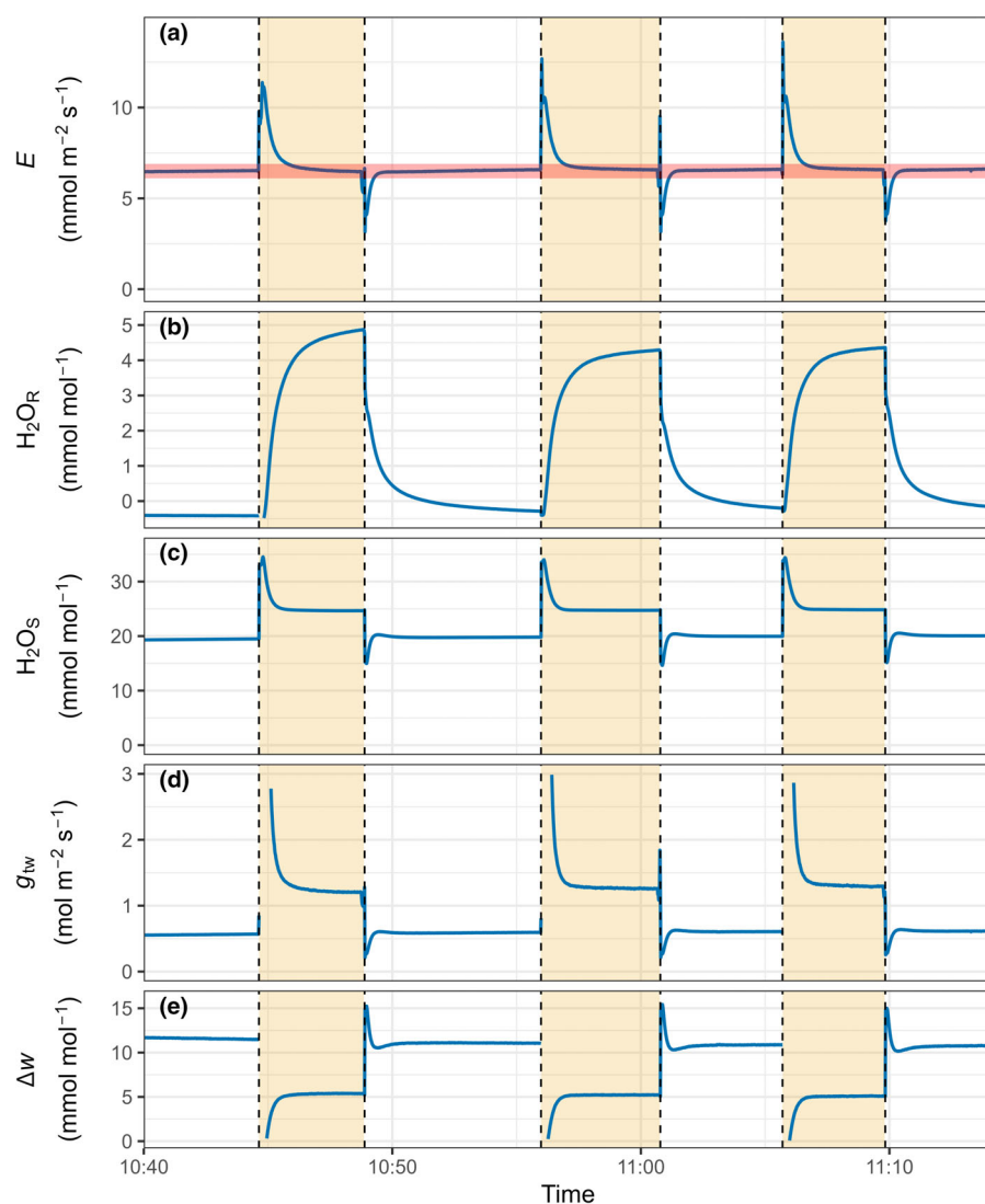
Fig. 1 Illustration of changes in gas exchange parameters during a series of successive changes of the carrier gas back and forth between nitox (unshaded regions) and nitox (yellow-shaded regions), in a leaf of Helianthus annuus . Calculated transpiration rate ( E , a) transiently increases upon each switch to helox, because changes in reference gas composition ( H_2O_R , b) cause a transient condition of nonsteady-state of sample gas composition ( H_2O_S , c), but transpiration quickly stabilizes, along with calculated total conductance to water vapor ( g_{tw} , d) and leaf-to-air water vapor mole fraction difference ( \Delta w , e; the equivalent vapor pressure gradient ( VPD_{leaf} ) in kPa is \Delta w/10 ). After the first switch to helox, the operator makes a small adjustment in the target flowrate for humidified air, and thus for reference vapor composition, to better balance the transpiration rates in helox and nitox, after which steady-state transpiration rate is virtually identical in helox and nitox during successive switches.
